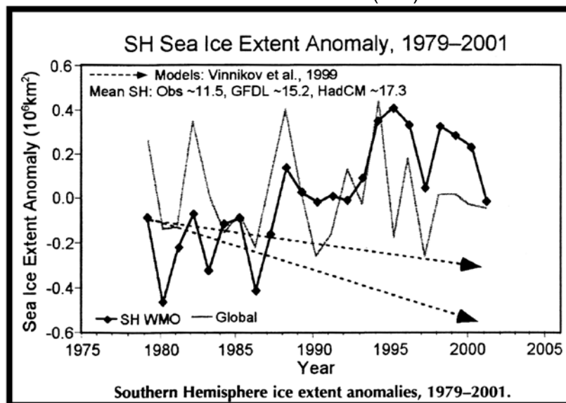
Sea Ice SH Hemisphere Predicted v. Observed (real)
