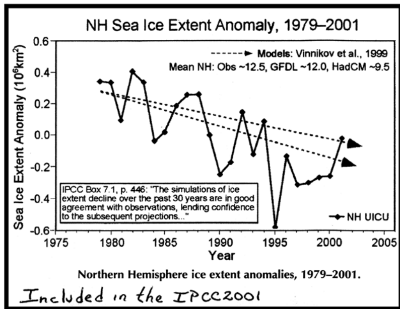
Sea Ice NH Hemisphere Predicted v. Observed (real)
