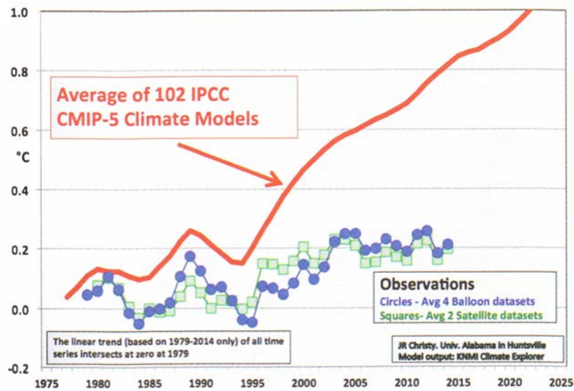
Global Temperatures - Predicted (red) v. Actual (blue & green)
